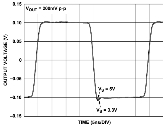
Figure 17. Small Signal Transient Response vs. Supply Voltage
