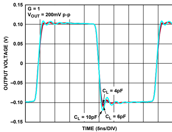
Figure 18. Small Signal Transient Response vs. Capacitive Load
